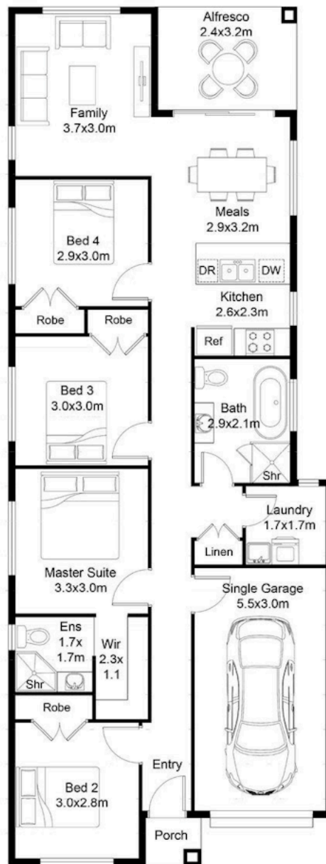
FLOOR PLAN
